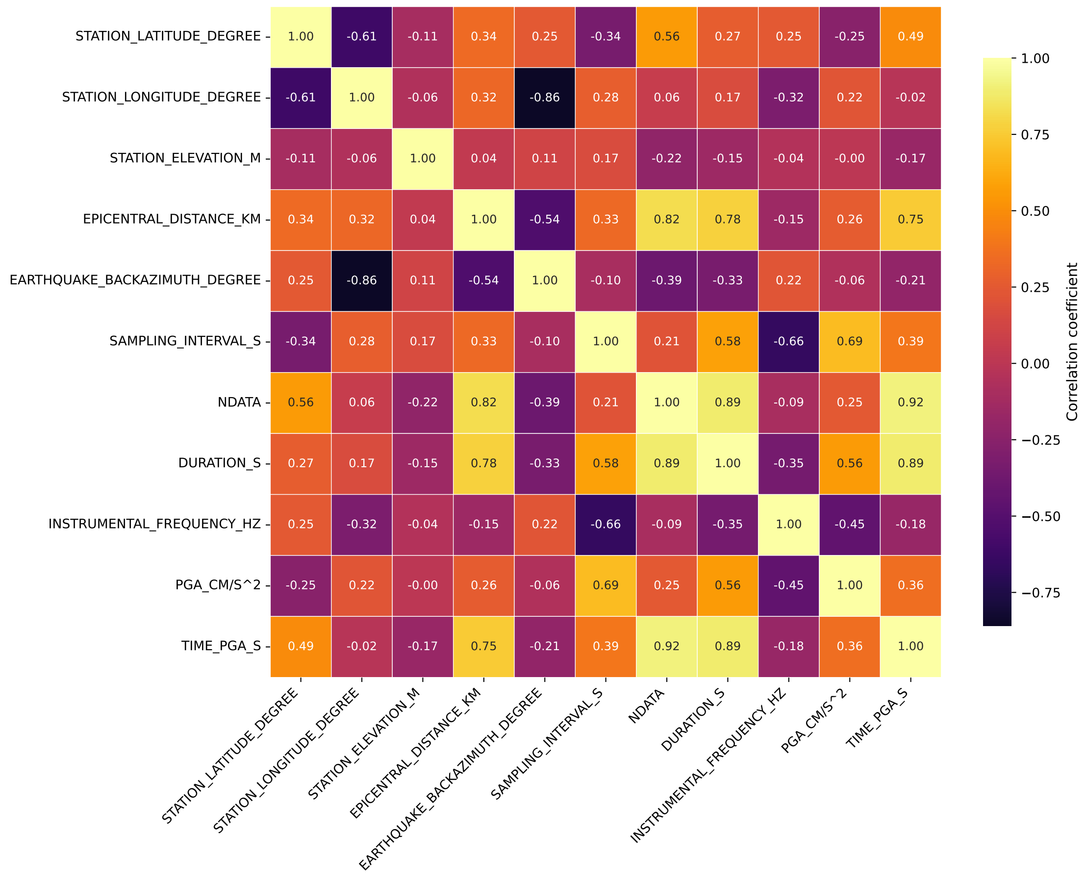
Correlation matrix — Far stations (178.5–421.4 km)
